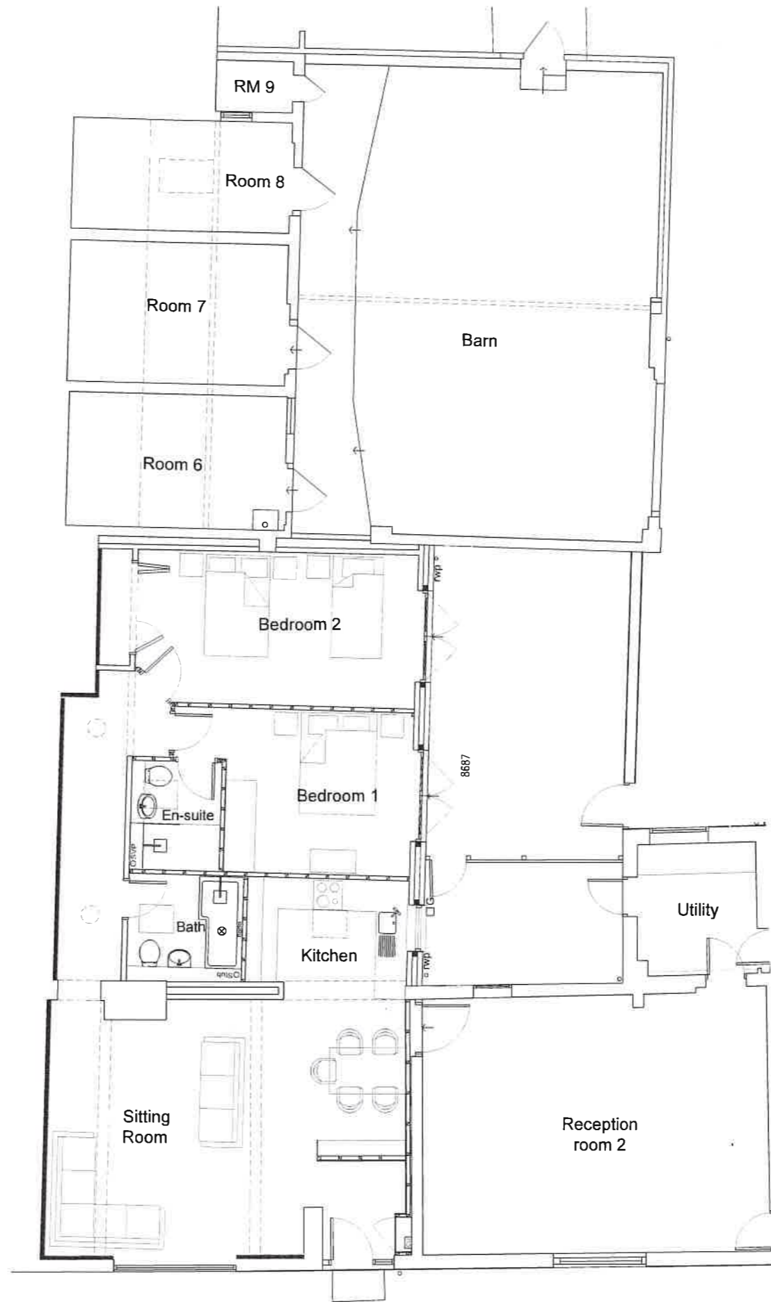
Ground Floor Plan Scale 1:50 @ A1
